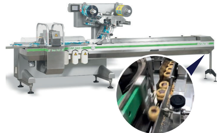
Wrapper FP095 complete with in-line feeding system and grouping-overlapping unit
